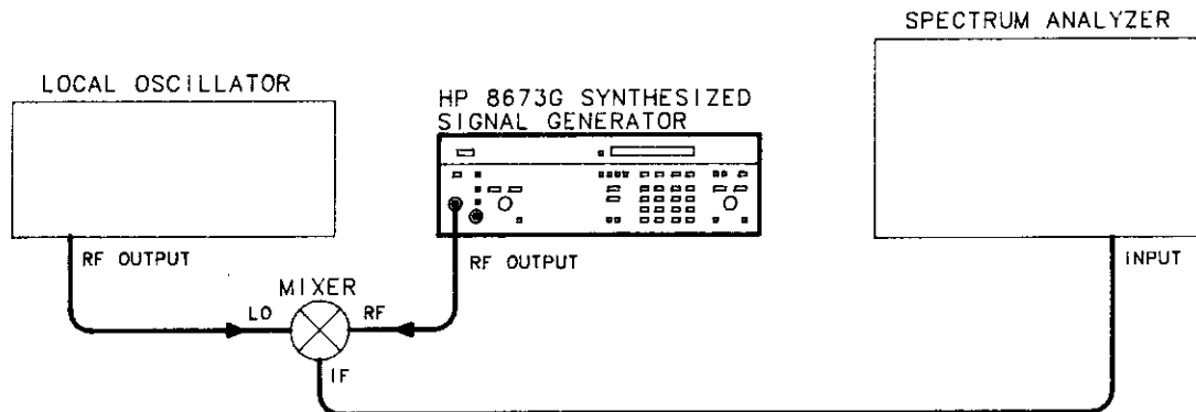
Figure 4-11. Single-Sideband Phase Noise Test Setup
