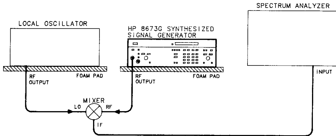
Figure 4-14. Power Line Related Spurious Signals Test Setup
