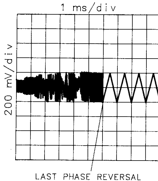
Figure 4-8. Frequency Switching Time Measurement Waveform
