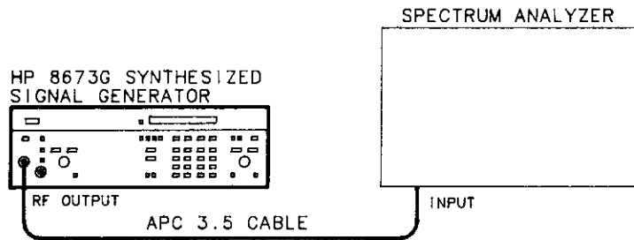
Figure 4-13. Non-harmonically Related Spurious Test Setup
